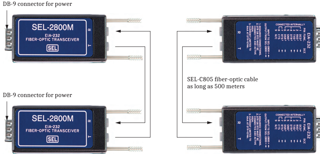
Figure 1 SEL-2800 Product Overview
